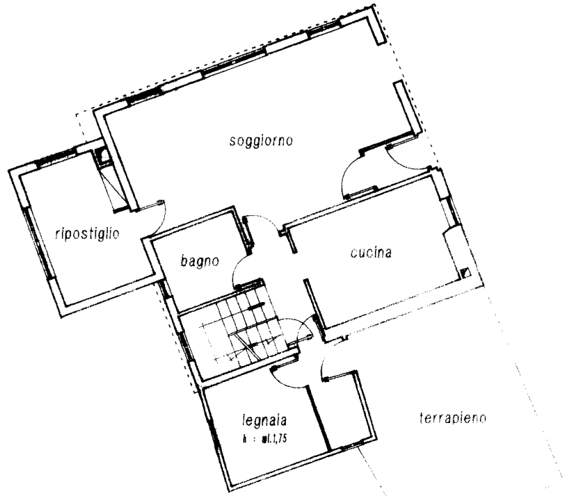
PIANO TERRA h=ml.2.15
