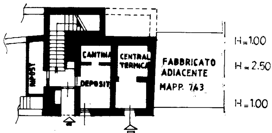
PIANO SEMINTERRATO
