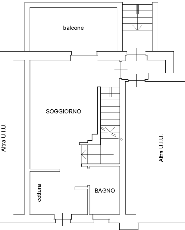
PIANO TERRA H = ml. 2,40
